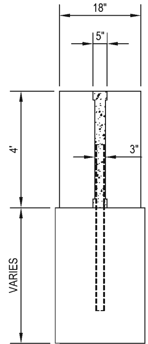
4' WALL SIDE ELEVATION
