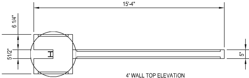
4' WALL TOP ELEVATION
