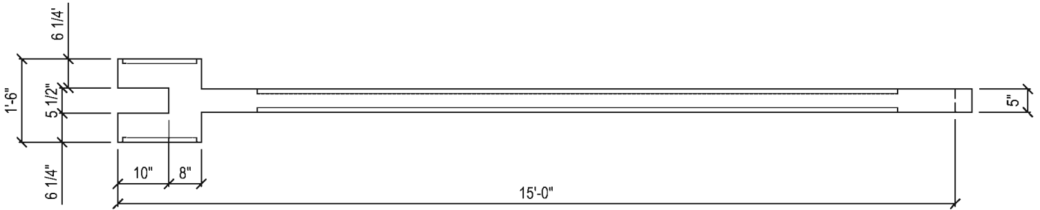
8' WALL TOP ELEVATION
