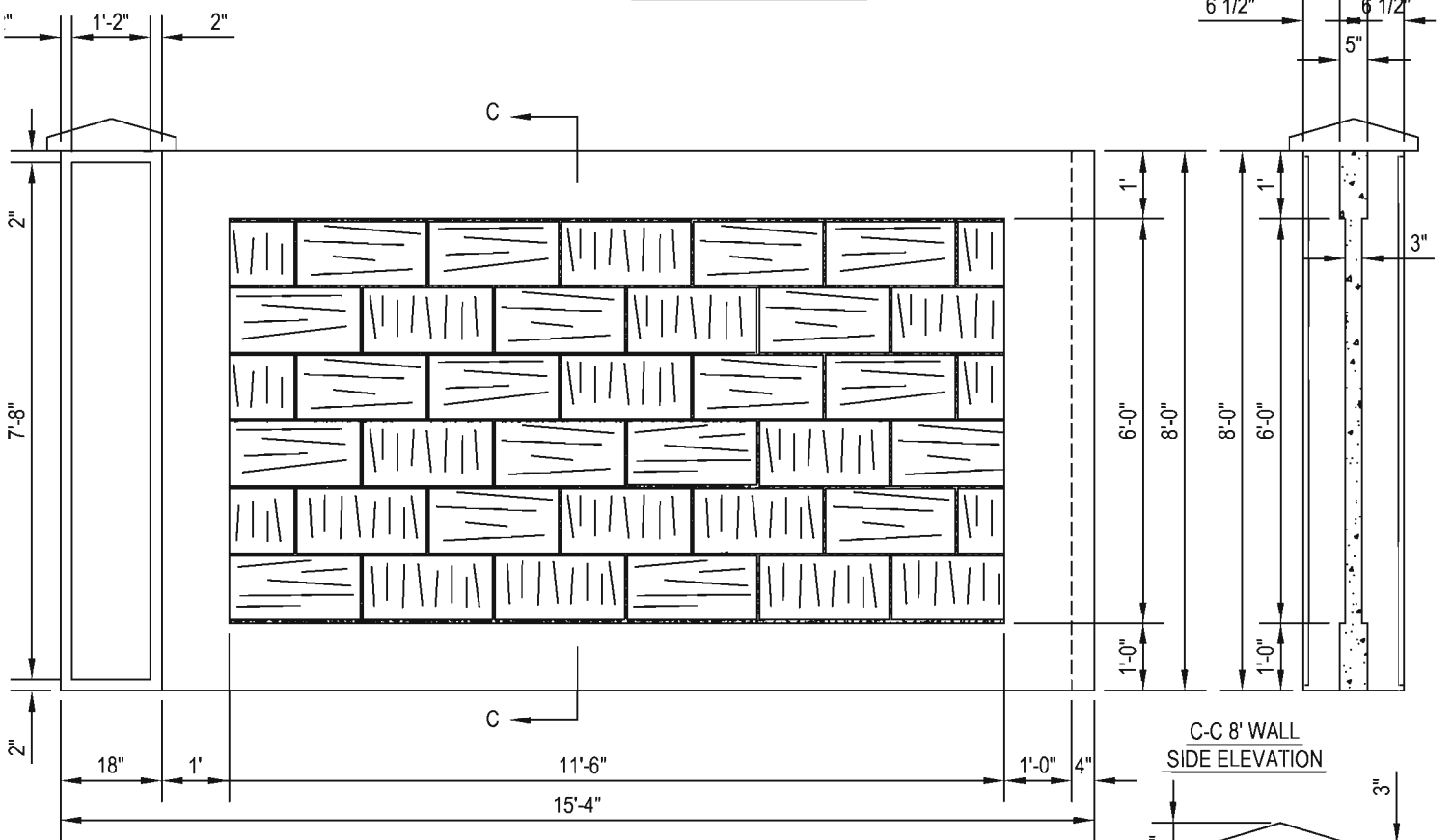
8' WALL ELEVATION
